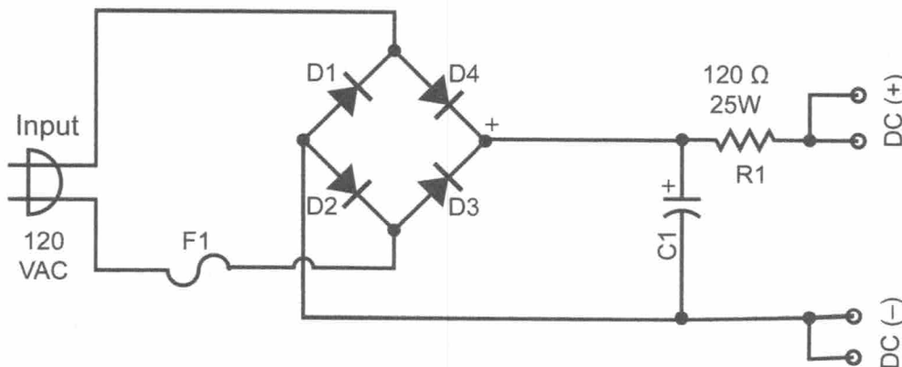
Figure 2 Schematic
