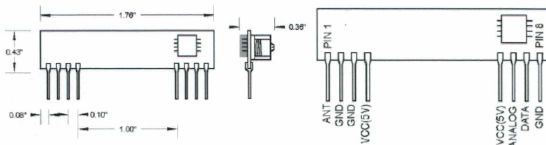
Mechanical Drawing
