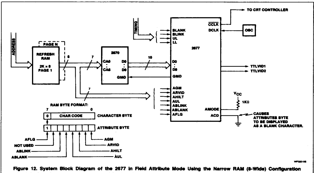
Figure 12. System Block Diagram of the 2677 in Field Attributes Mode Using the Narrow RAM (8-Wide) Configuration
